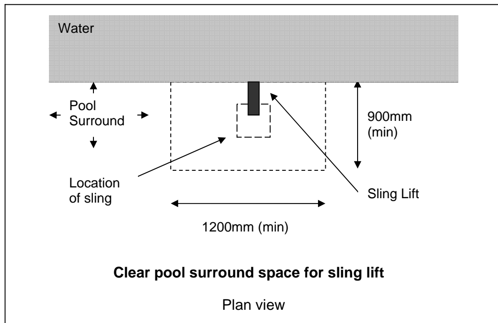
Figure D3.10 Clear pool surround space for sling lift
